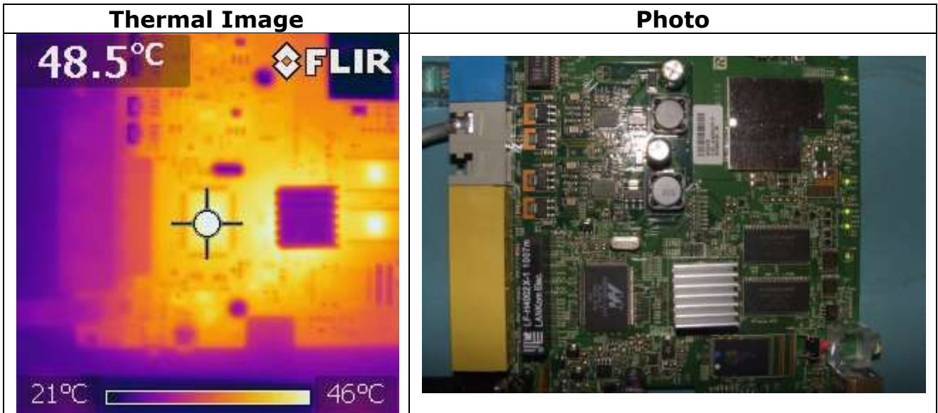
Figure 21: Thermal image of Linksys WRP400-G4 router (image 1)
